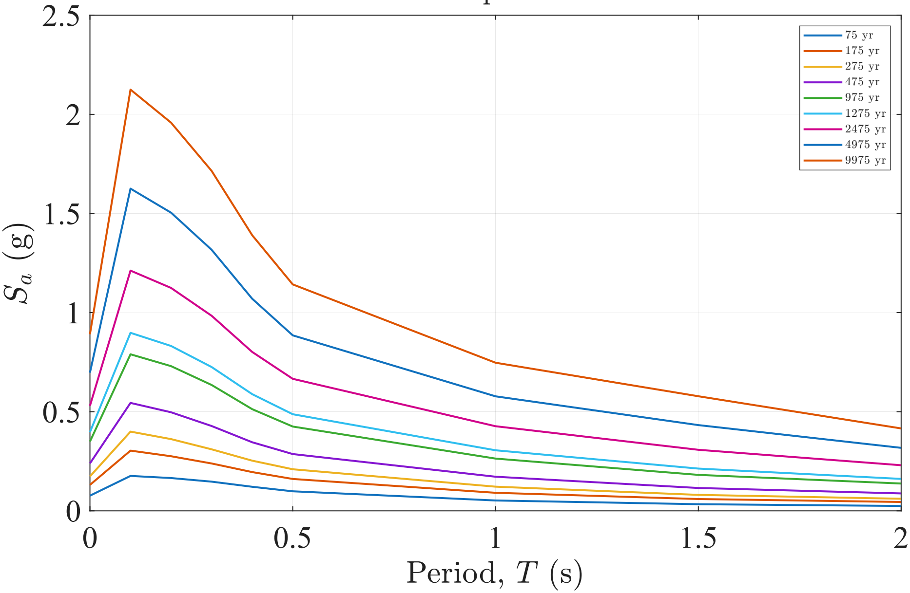
Uniform Hazard Spectrum - Guwahati
